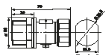
P8AX_716/NF
