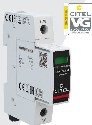
DAC50VGS-10
