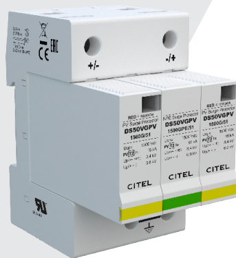
DS50VGPV-1500G/51
