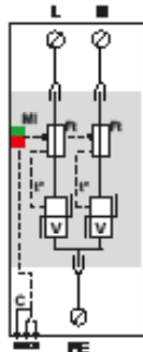
DAC40CS-20
