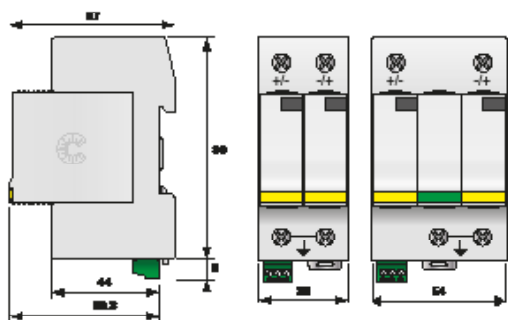
DS50PVS-500/51 DS50PVS-800G/51
