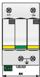
DS50VGPVS-G/12KT1
