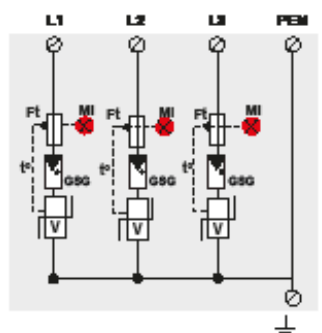
DUT250VG-300/TNC
