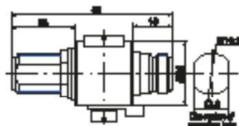
P8AX_N/FF
